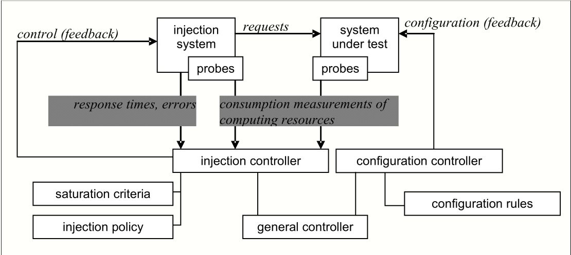
figure 6. Autonomous benchmarking: self-optimization of a system under test and autonomic search of performance saturation
