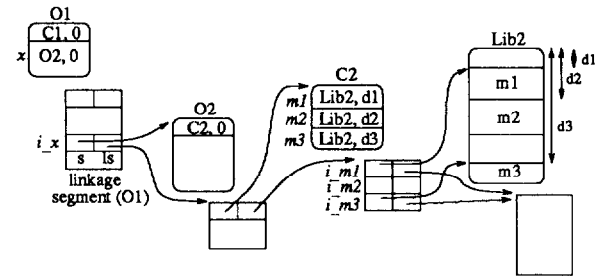
Figure 3: Object binding and method call
